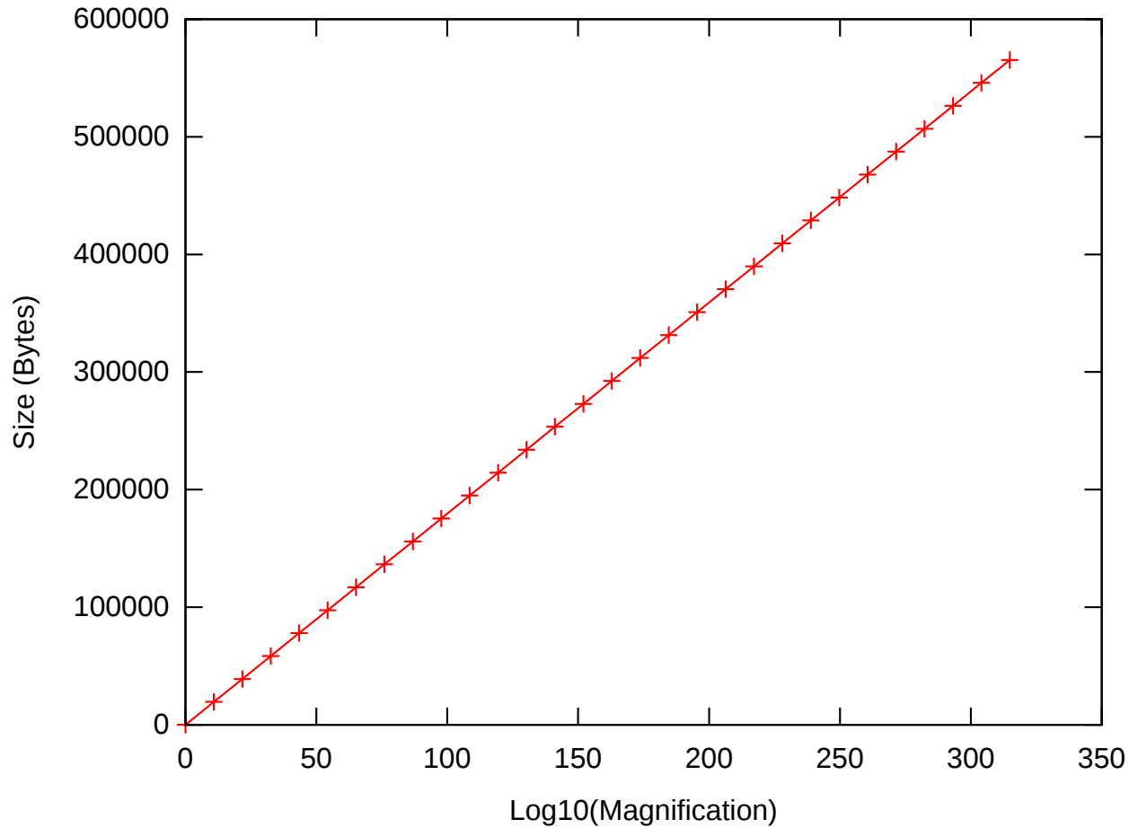
Memory Usage Per Rational
