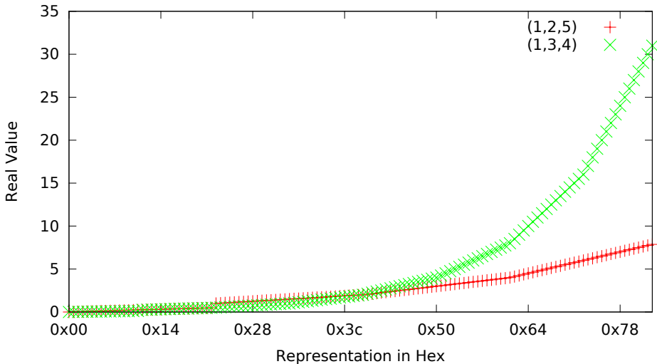
8 Bit Floats (s,e,m)
