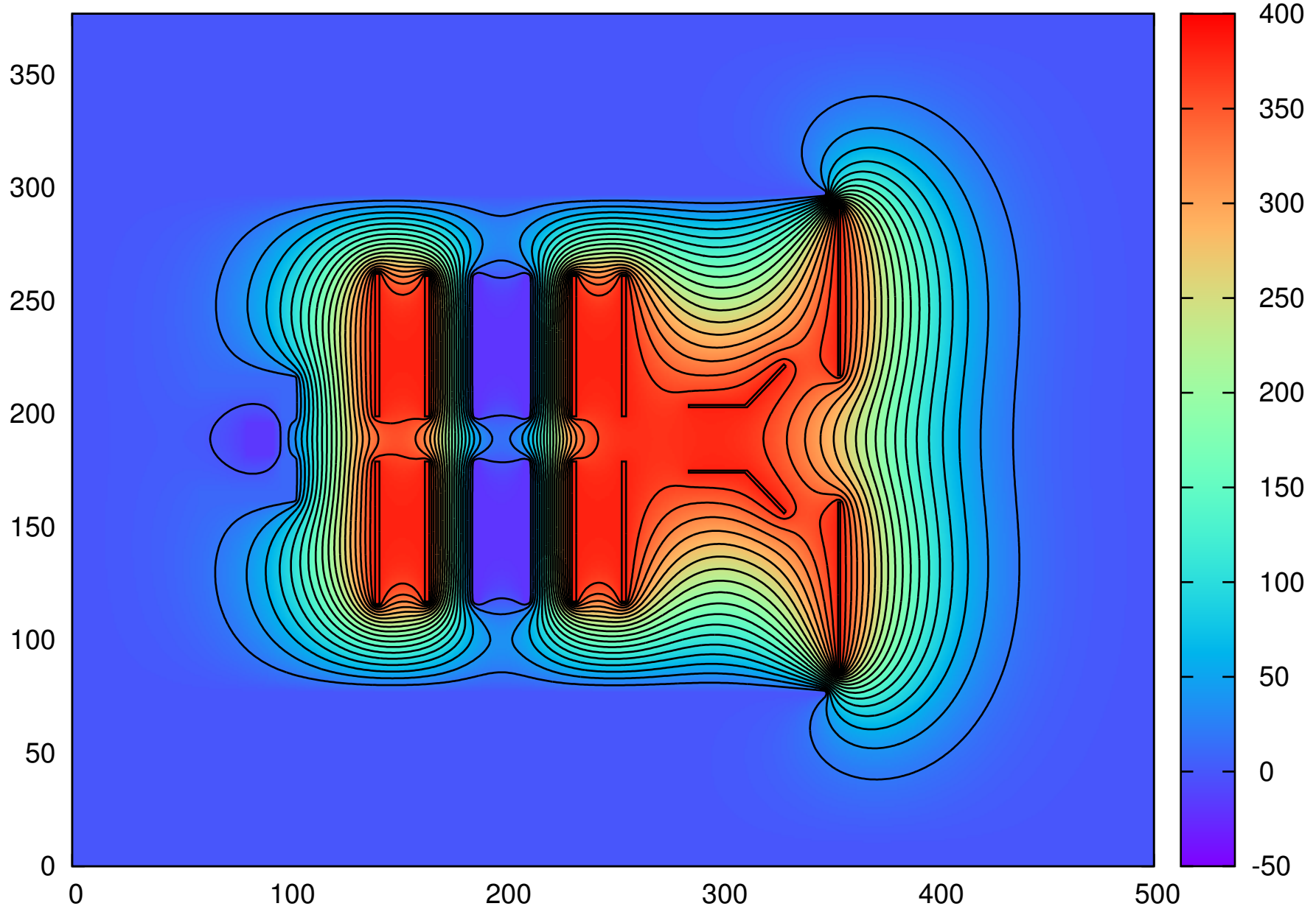
TCS Electron Gun
