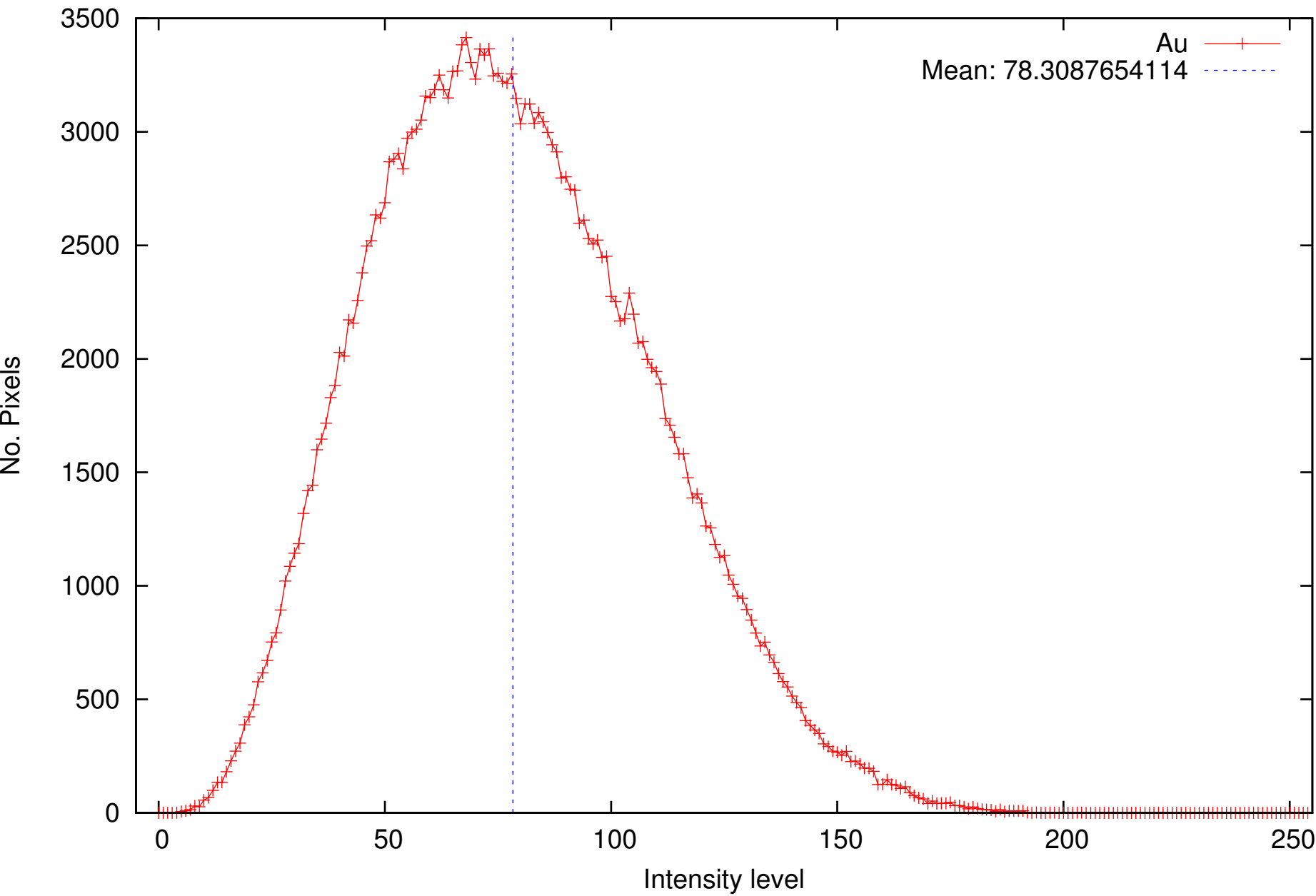
Intensity level distributions of Au SEM image
