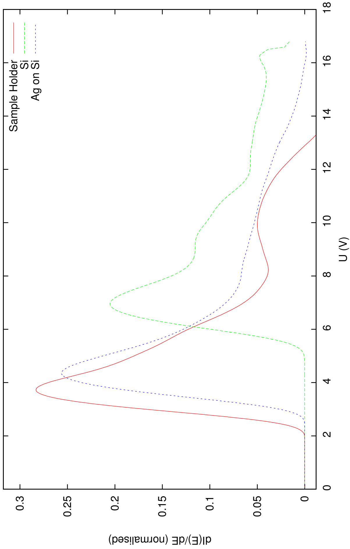
Comparison of S(E) curves for: Sample Holder (Stainless Steel), Si and Ag on Si
