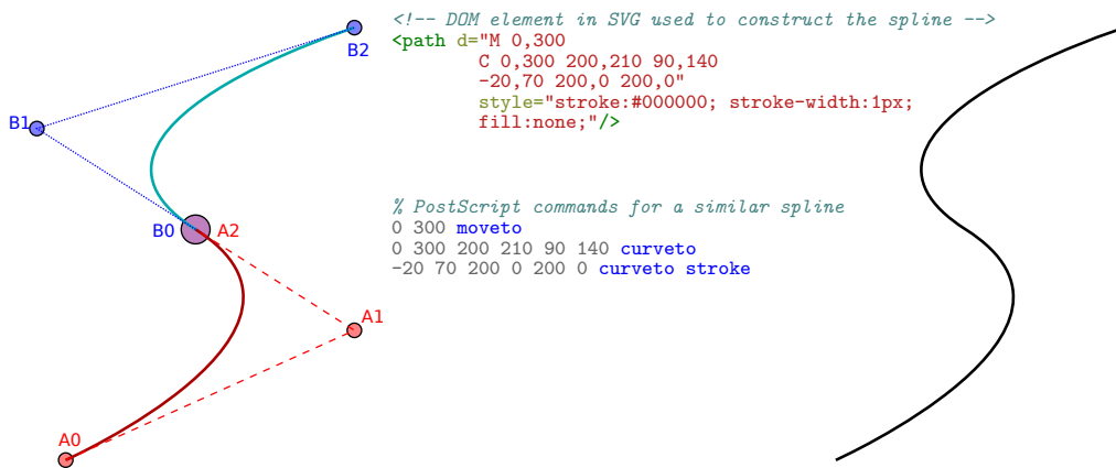
Figure 3.4: Constructing a Spline from two cubic beziers (a) Showing the Control Points (b) Representations in SVG and PostScript (c) Rendered Spline
