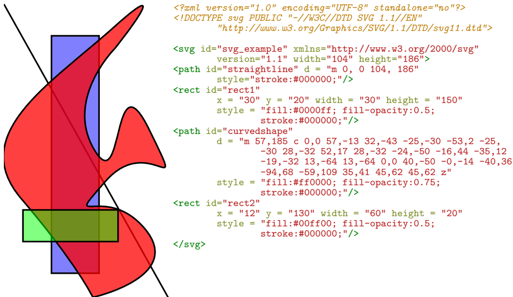
Figure 3.4: Vector image and a possible SVG representation
