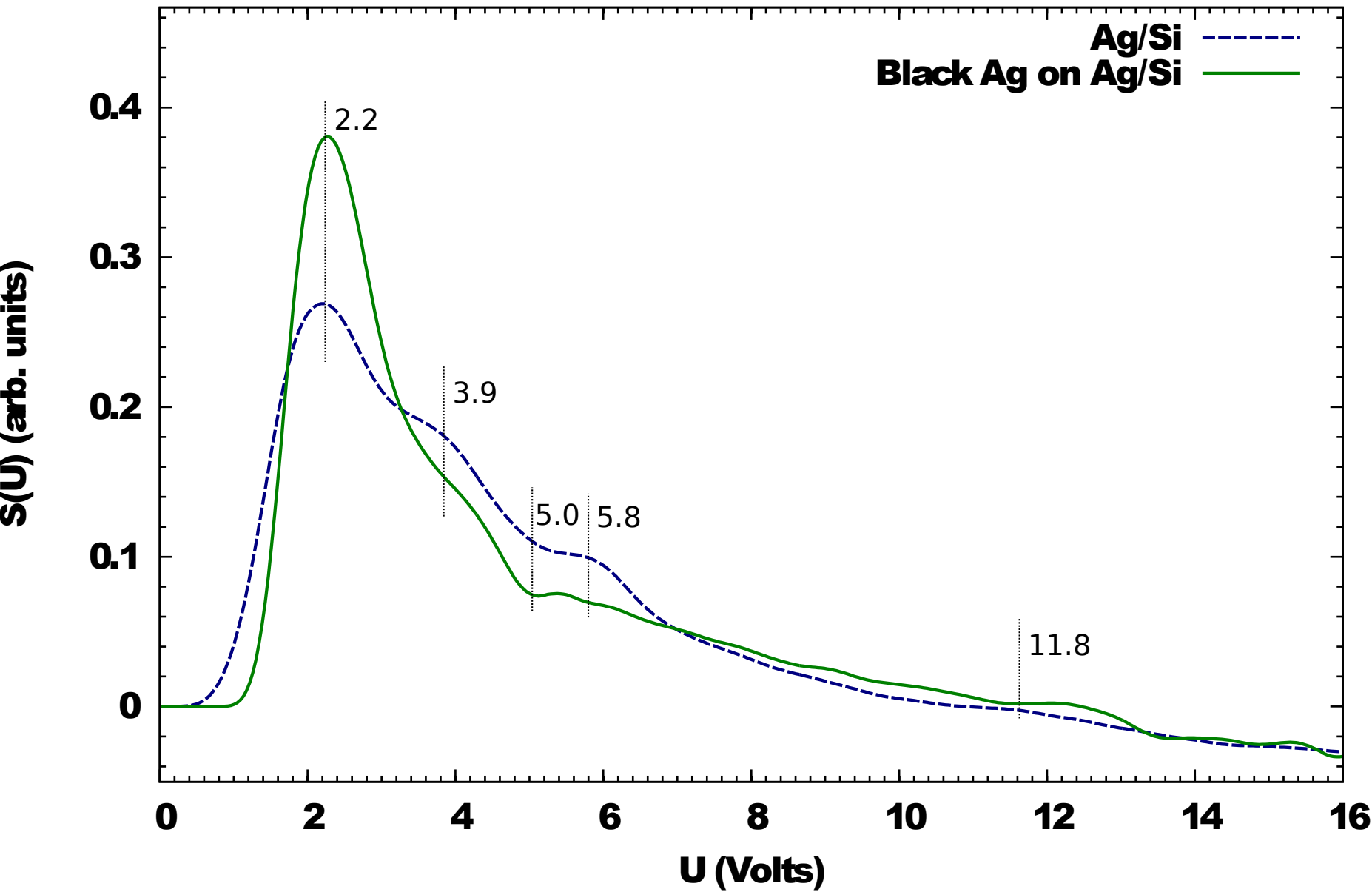
S(U) curves for Ag/Si .vs. Black Ag on Ag/Si
