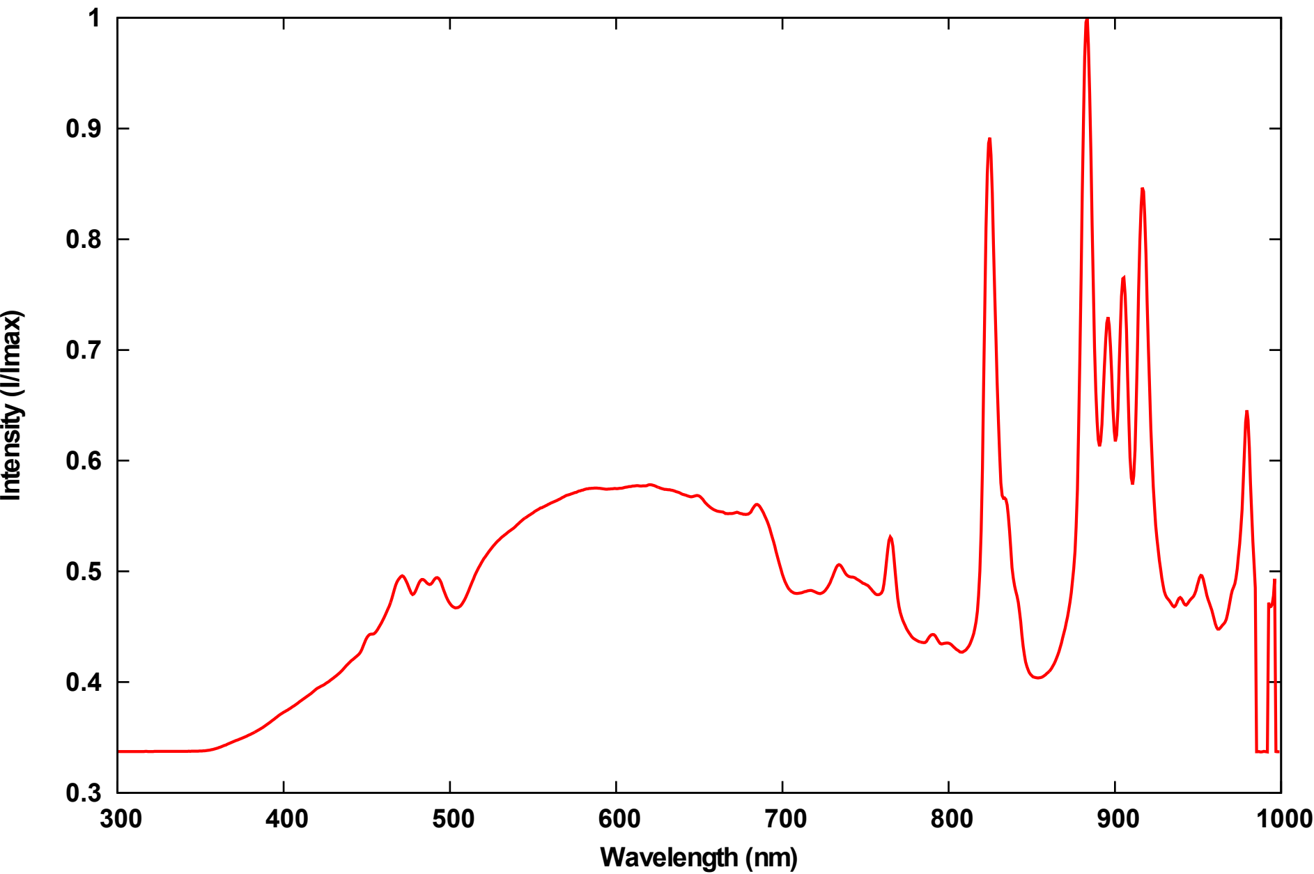
Spectrum of Xe arc lamp
