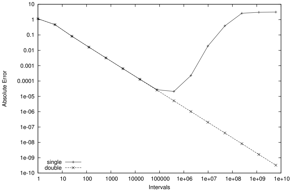
Calculations of PI using Numerical Integration (Simpson Method)
