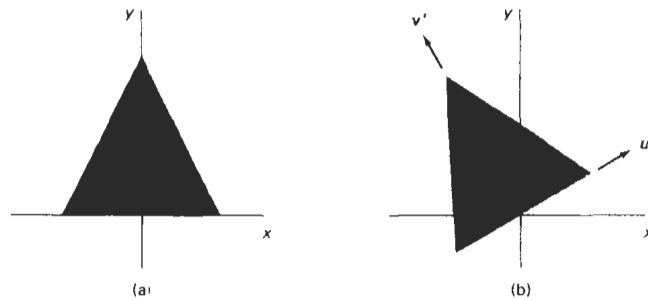
Figure 5-14 The rotation matrix for revolving an object from position (a) to position (b) can be constructed with the values of the unit orientation vectors \mathbf{u}' and \mathbf{v}' relative to the original orientation.
