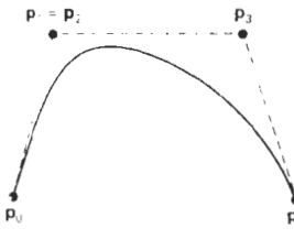
Figure 10-36 A Bézier curve can be made to pass closer to a given coordinate position by assigning multiple control points to that position
