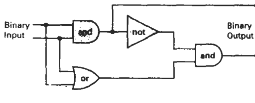
Figure 7-6 Model of a logic circuit.
