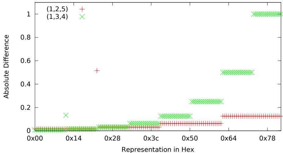
Difference Between Successive 8 bit Floats (s,e,m)
