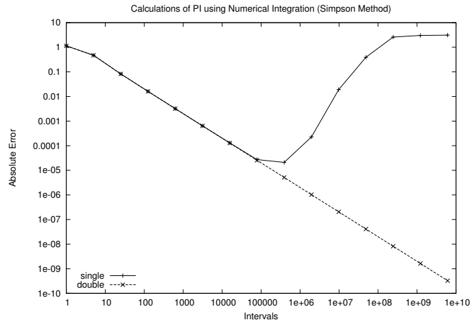
Figure 3.10: Numerical calculation of \pi
