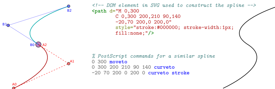
Figure 2.4: Constructing a Spline from two cubic Béziens (a) Showing the Control Points (b) Representations in SVG and PostScript (c) Rendered Spline
