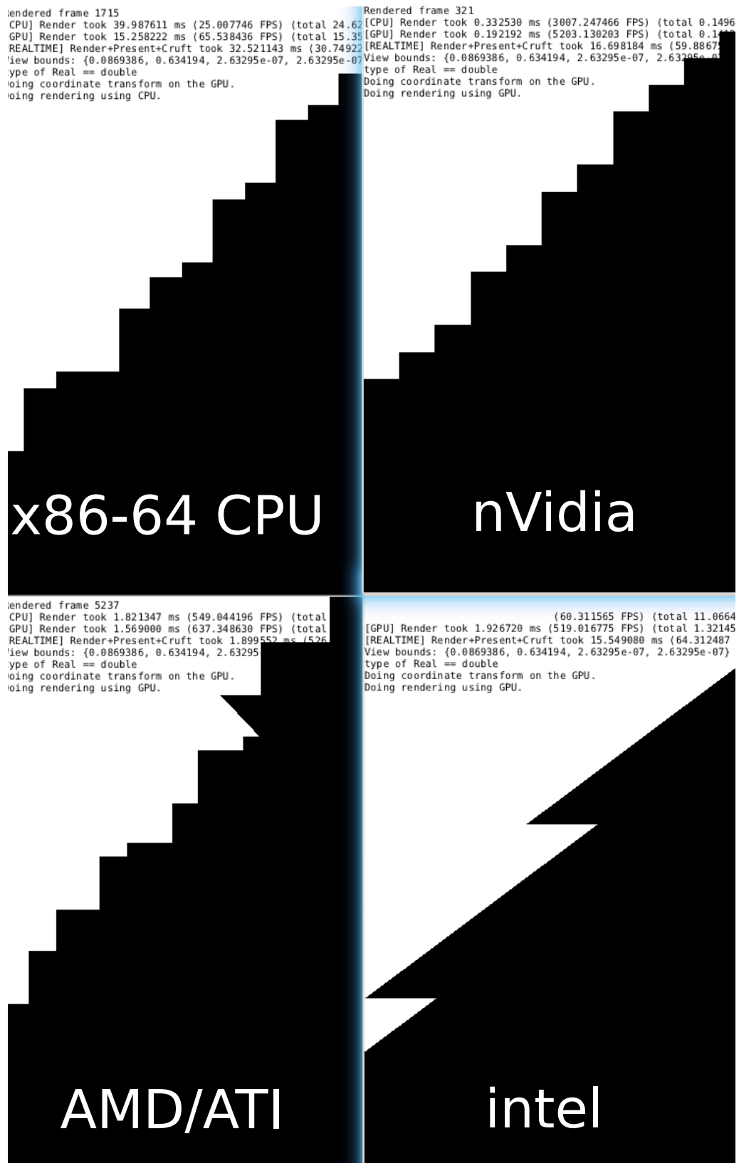
Figure 2.12: CPU and GPU evaluation of x^2 + y^2 < 1 at \approx 10^6 magnification
