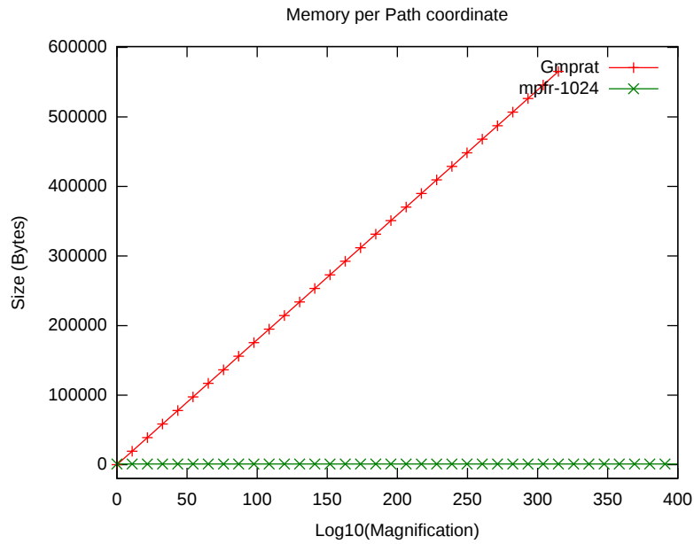
Figure 4.7: Memory used per Path coordinate whilst zooming in
