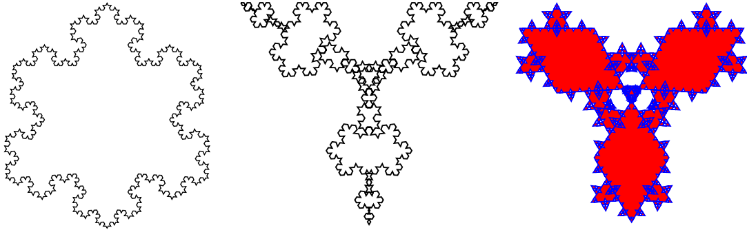
Figure 2.9: Koch “snowflakes” generated using Javascript to modify an SVG DOM. The interactive HTML5 document can be found at http://szmoore.net/ipdf/sam/figures/koch.html
