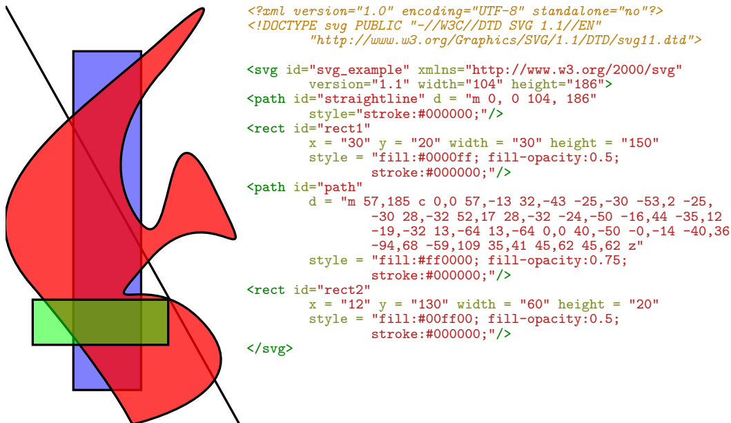
Figure 3.4: A vector image demonstrating some ideas from Section 3.2 and its representation in SVG
