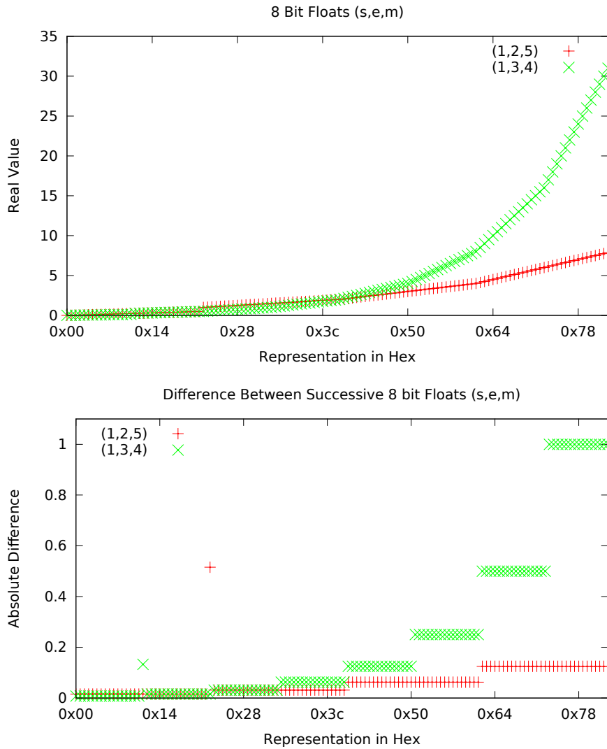
Figure 3.5: The mapping of 8 bit floats to reals
