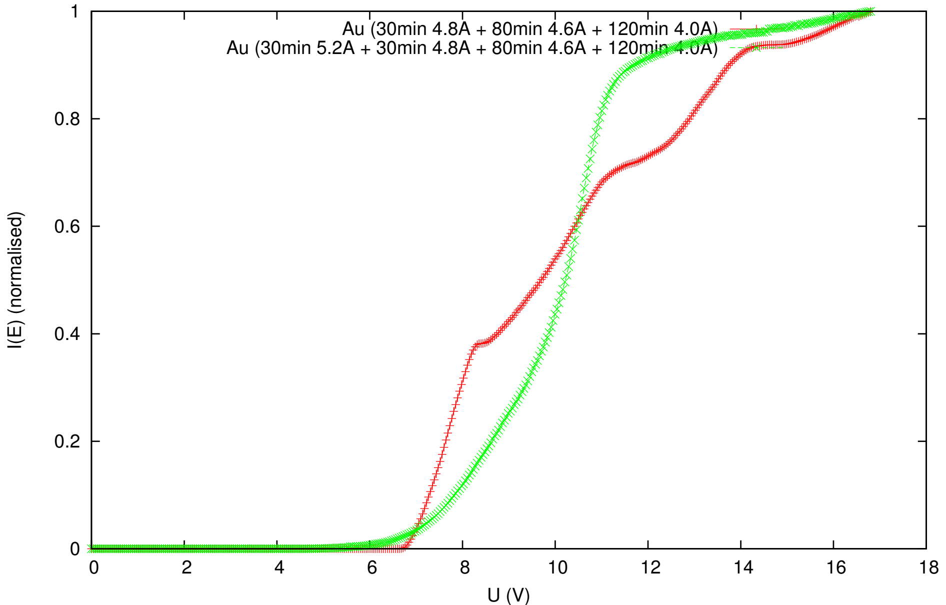
Time Evolution of Au on Si I(E) curves Focus not altered between curves; different focus to set1
